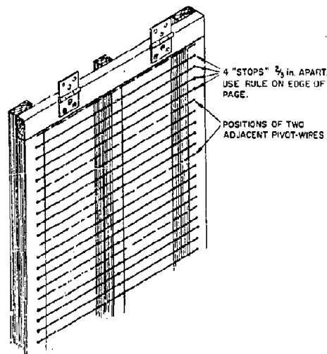
Fig. B-11. Attaching flap stops.
